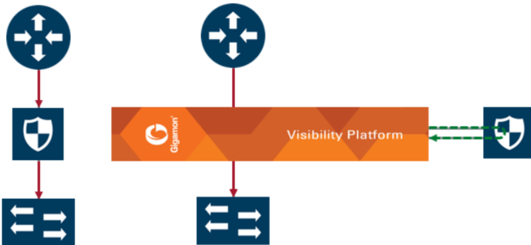
Figure 42 Simple Inline Tool Arrangement
