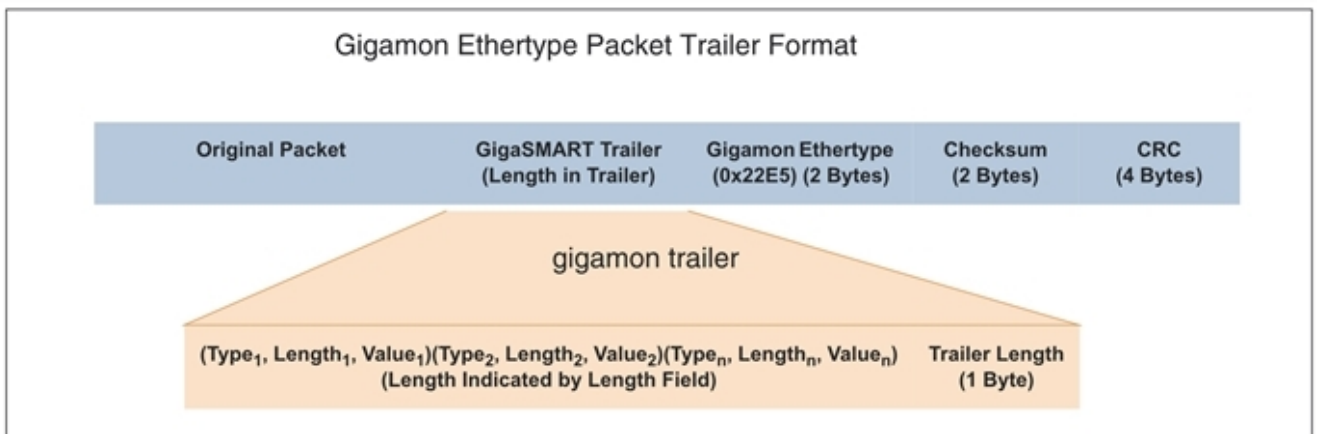
Figure 157 GigaSMART Trailer Format
