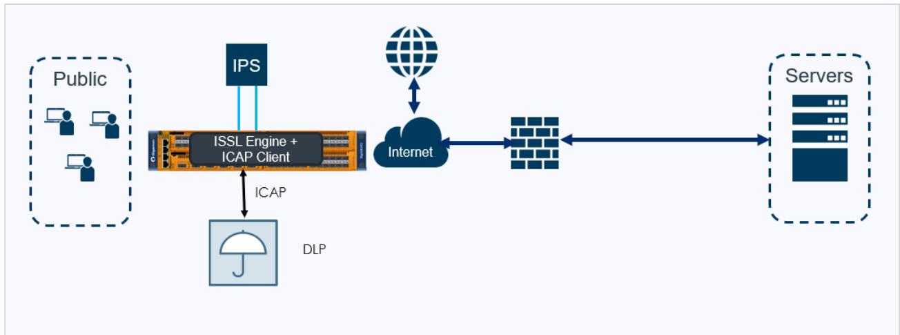
Figure 18 Inline SSL Solution with ICAP Client support – Outbound Deployment
