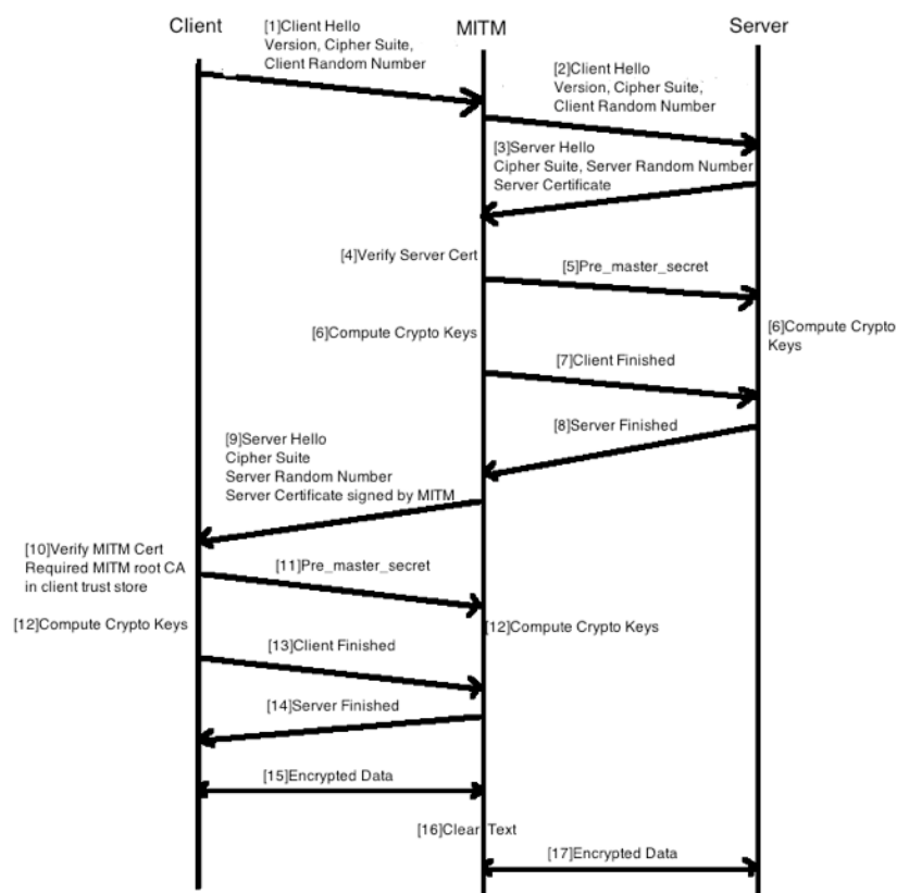
Figure 36 Man-in-the-Middle TLS/SSL Handshake
