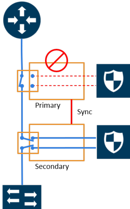
Figure 22 Traffic Flows Through Node with Secondary Role after Primary is Lost
