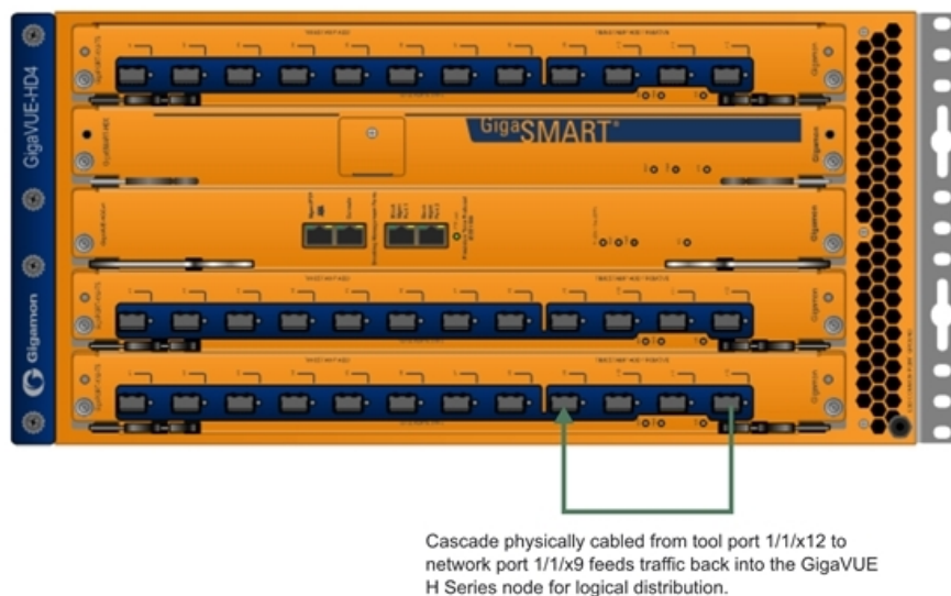
Figure 155 Cascade Physically Cabled from Tool to Network Port
