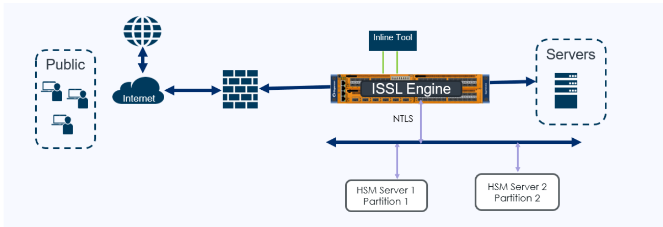
Figure 82 iSSL with Thales Luna - Inbound support
