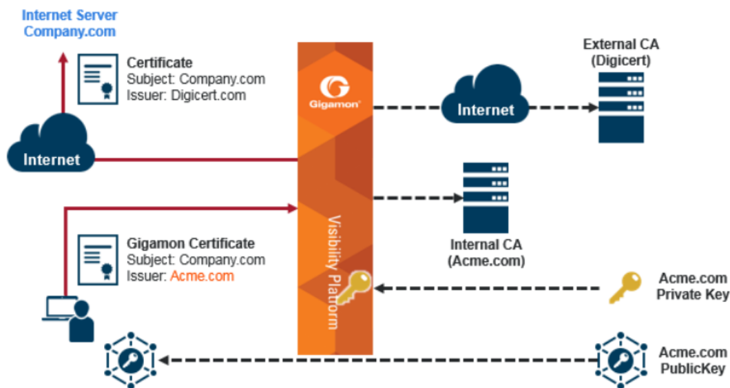
Figure 38 Outbound Deployment of Inline TLS/SSL Decryption
