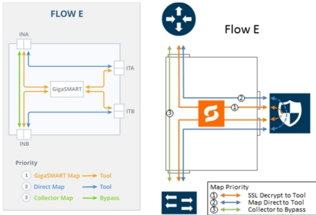
Figure 58 FLOW E Views
