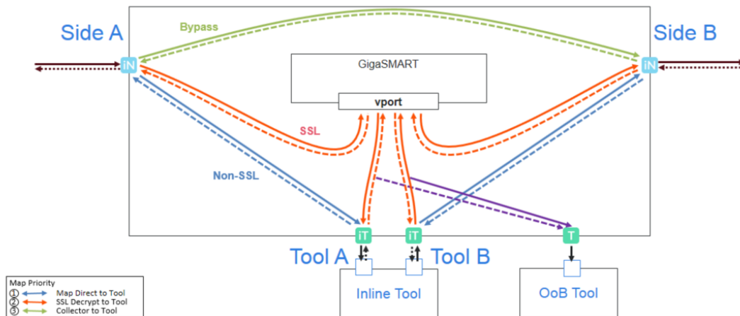
Figure 48 Packet Flow for Inline SSL Decryption
