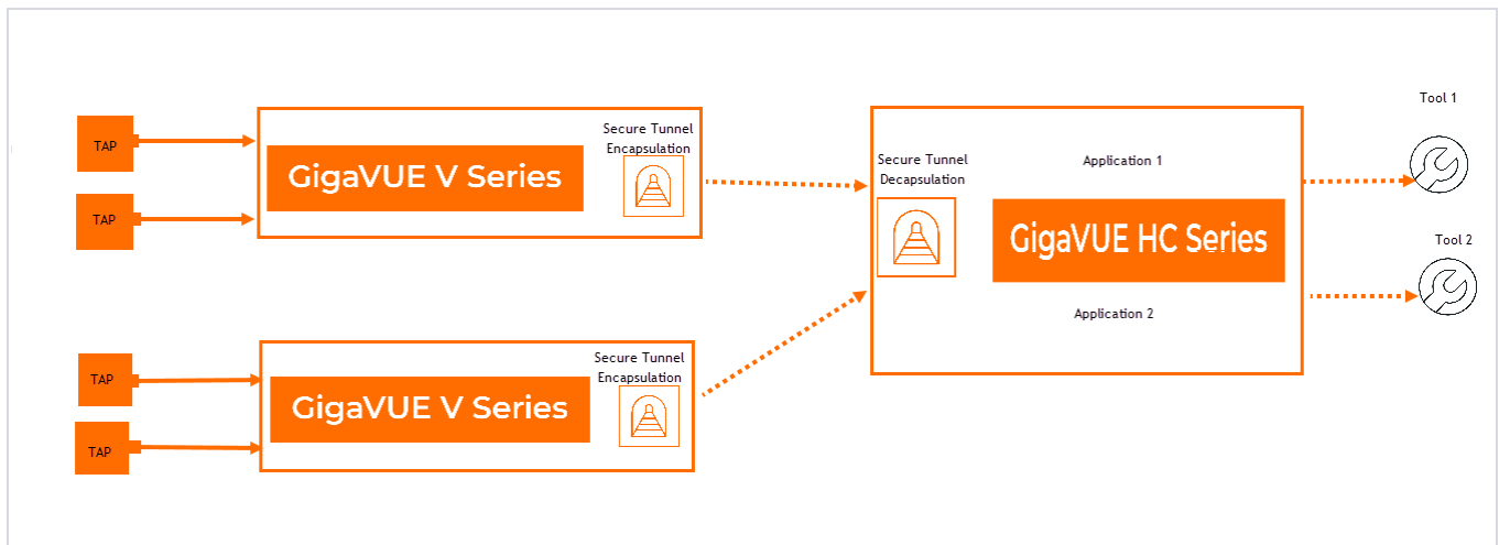
Figure 139 GigaVUE HC Series with a single IP Interface and multiple Map rules
