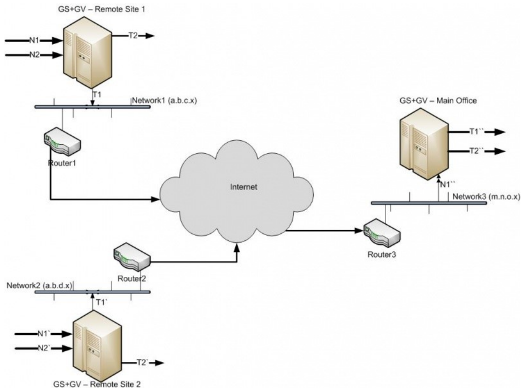
Figure 128 L2GRE Tunnel Encapsulation/Decapsulation
