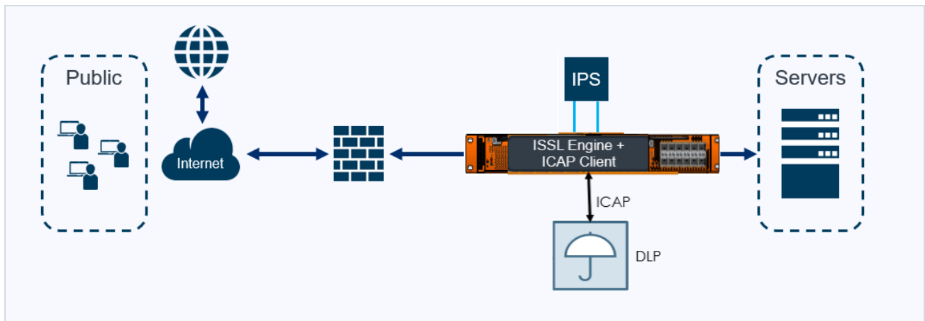
Figure 19 Inline SSL Solution with ICAP Client support – Inbound Deployment
