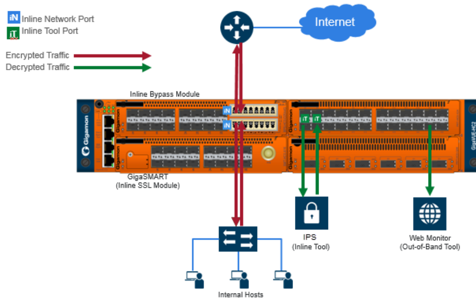
Figure 47 GigaVUE Modules: GigaSMART and Inline Bypass
