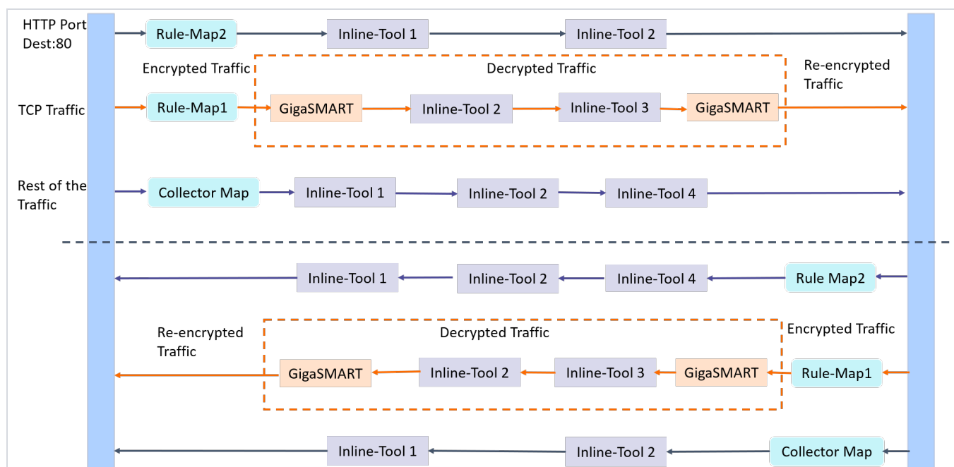
Figure 15 Flexible Inline Decryption Solution
