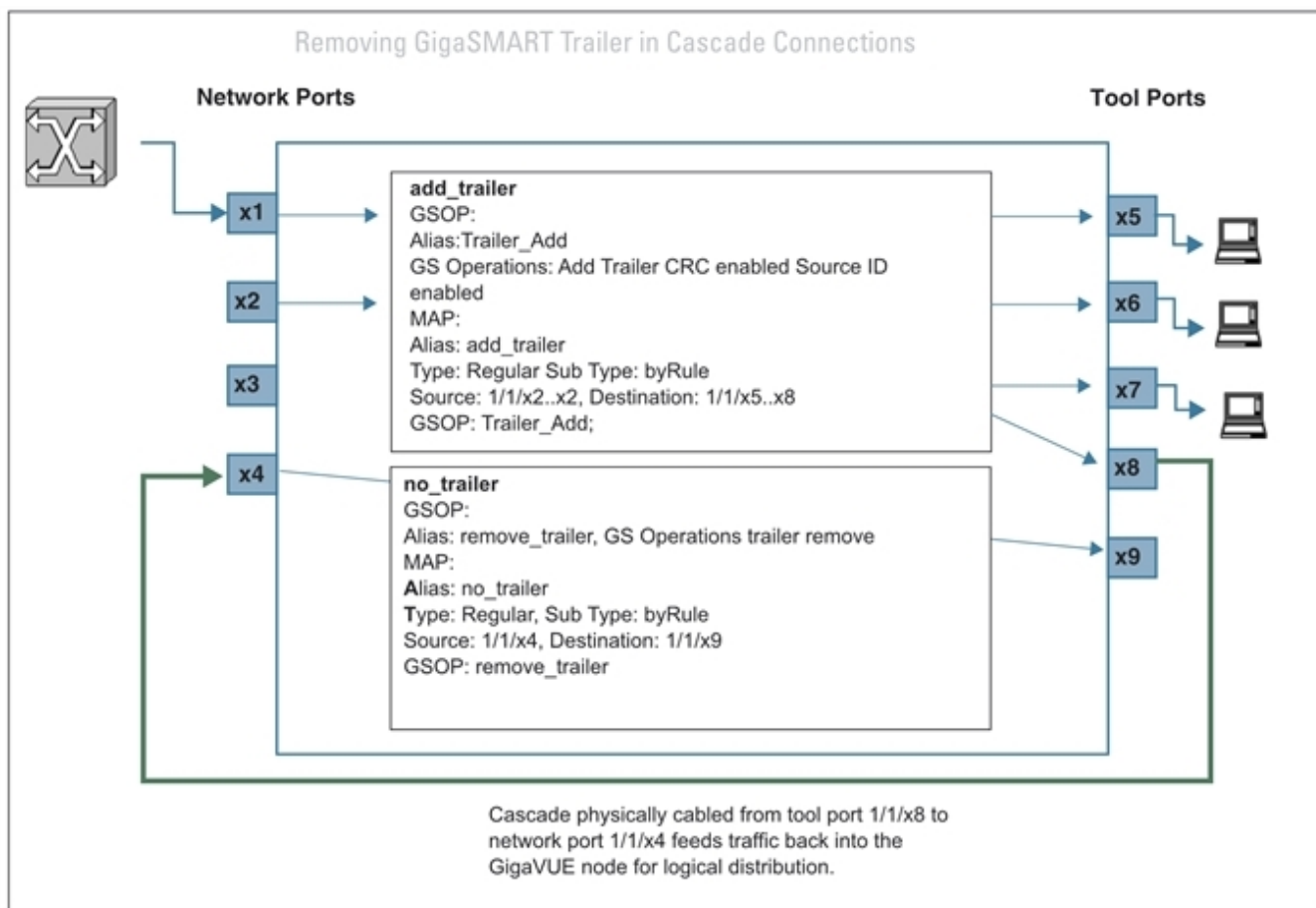
Figure 156 Removing the GigaSMART Trailer from a Cascade Connection
