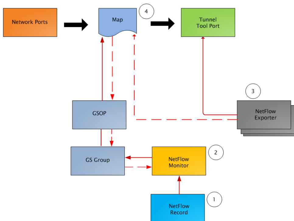
Figure 118 NetFlow Generation Components
